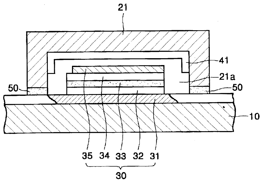
FIG. 1 (PRIOR ART)
